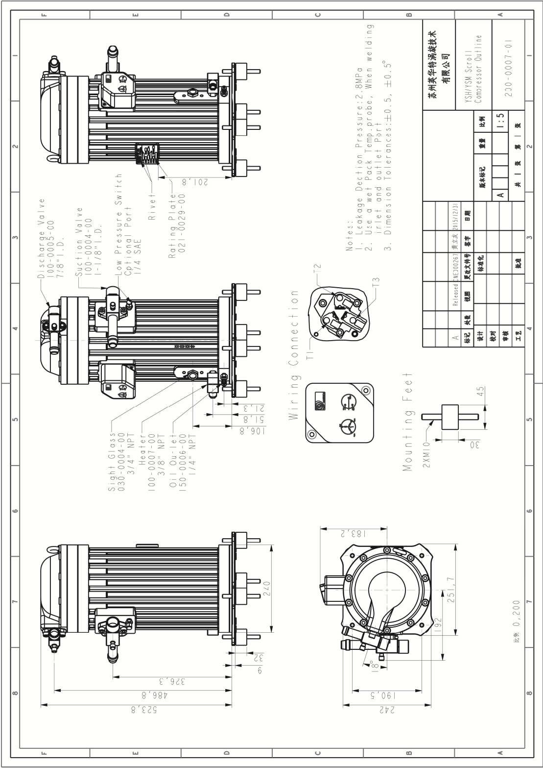
*10 压缩机外形图 Compressor Outline Dimensions
