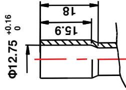
Detail of Discharge Tube
